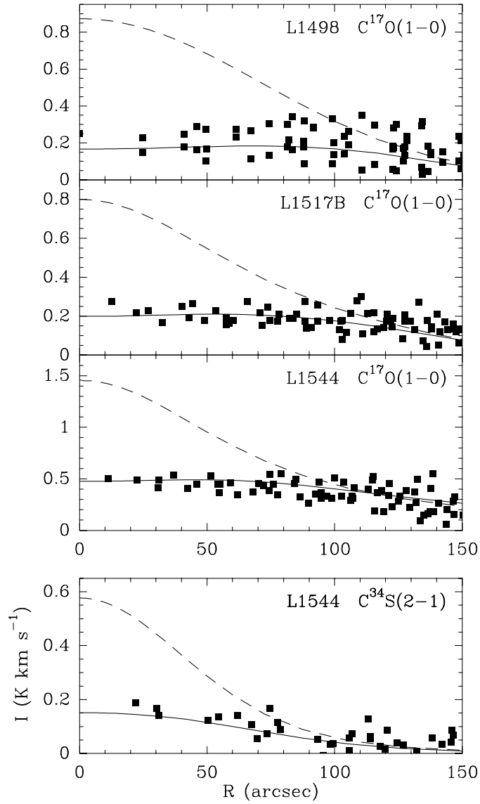
FIG. 4.— Radial profiles of integrated emission for \text{C}^{17}\text{O}(1-0) (three top panels) and \text{C}^{34}\text{S}(2-1) (bottom panel) toward selected cores. Observations are indicated by solid squares and results from radiative transfer models are indicated by lines. The models assume the same abundance profiles as those in Fig. 3, with the ISM isotopic ratio of 3.65 for \text{C}^{18}\text{O}/\text{C}^{17}\text{O} (Penzias 1981) and the Solar ratio of 22.7 for \text{C}^{32}\text{S}/\text{C}^{34}\text{S} . Note how the constant abundance models (dashed lines) miss the data toward the core centers by large factors. The models with central abundance drops (solid lines), in contrast, automatically fit the data without adjusting any additional parameter.
